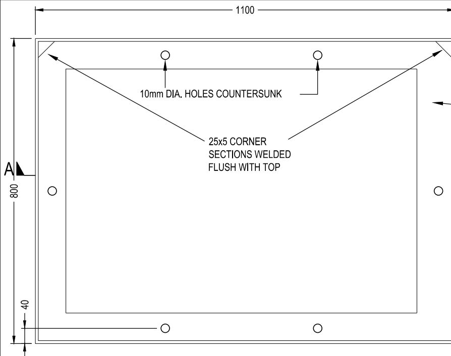
FRAME SCALE 1:10
