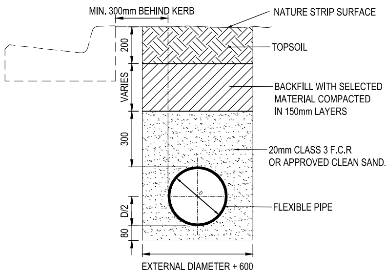
FLEXIBLE PIPE BEDDING DETAIL
