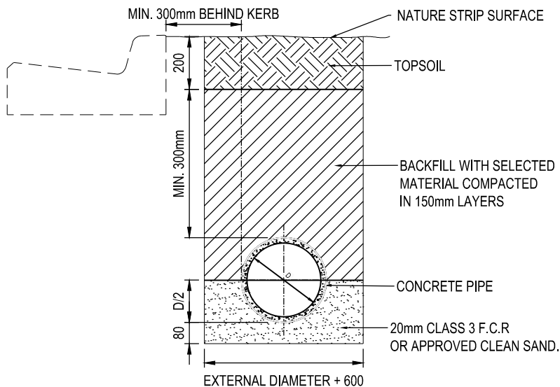
CONCRETE PIPE BEDDING DETAIL
